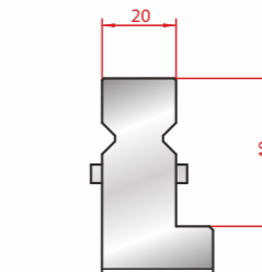
Wila New Standard Punch
